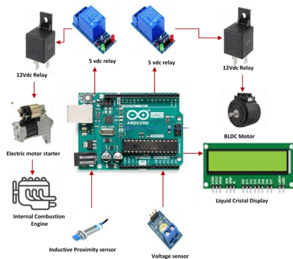
Fig. 9. Block diagram
